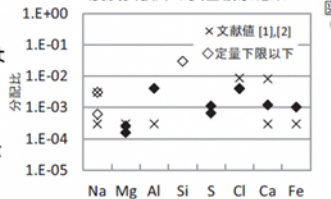
図3 FP共存条件での不純物成分の分配比 [1]Data of Inorganic Solvent Extraction (1) JAERI1047 [2]PUREX Technical Manual (1980)
